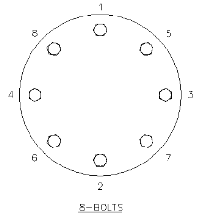
Figure 'B' EXAMPLE OF BOLT TORQUE SEQUENCE
