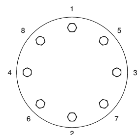
Figure 'B' EXAMPLE OF BOLT TORQUE SEQUENCE
