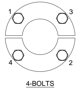
FIGURE 'D' EXAMPLE OF BOLT TORQUE SEQUENCE
